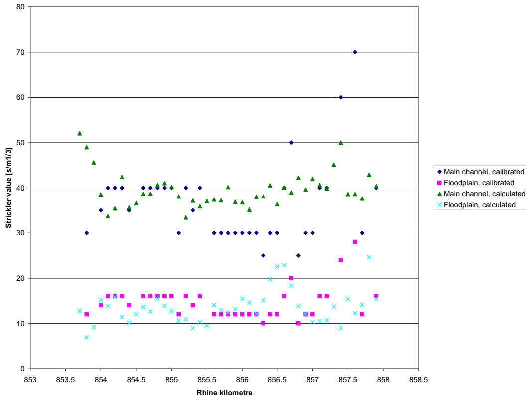
Figure 5-3: Calibrated and calculated Strickler values in main channel and floodplain
