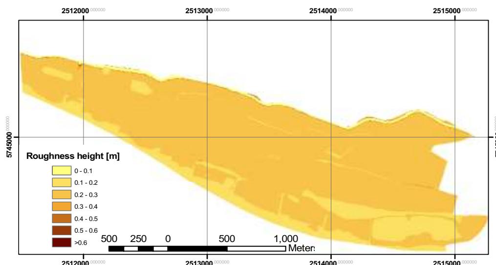
Figure 5-19: Roughness distribution over the floodplain, grassland coverage (see section 3.2), HHQ of 1995
