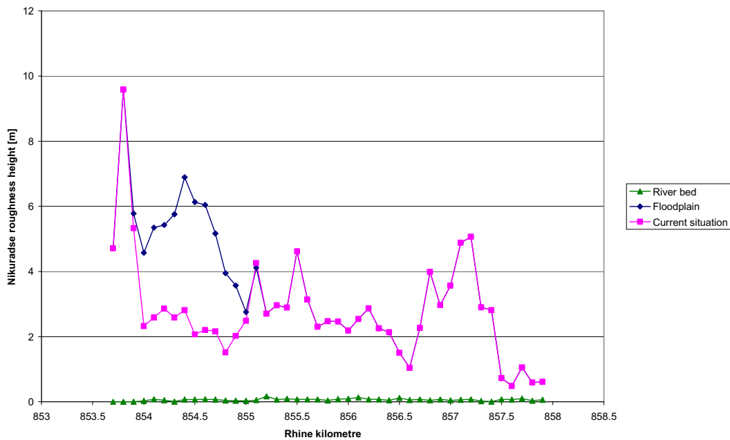
Figure 5-10: Roughness heights for each cross-section, forestation behind the second summer dike (see section 3.2), HHQ of 1995
