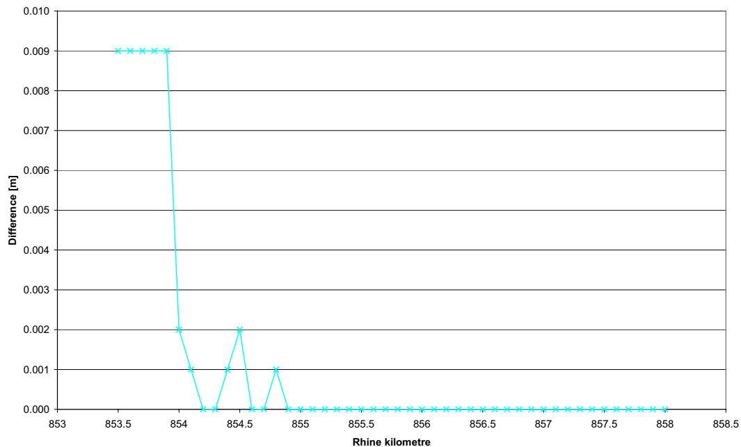
Figure 5-14: Differences in HHW between a scenario with forestation in clusters between both summer dikes (see section 3.2) and the current situation
