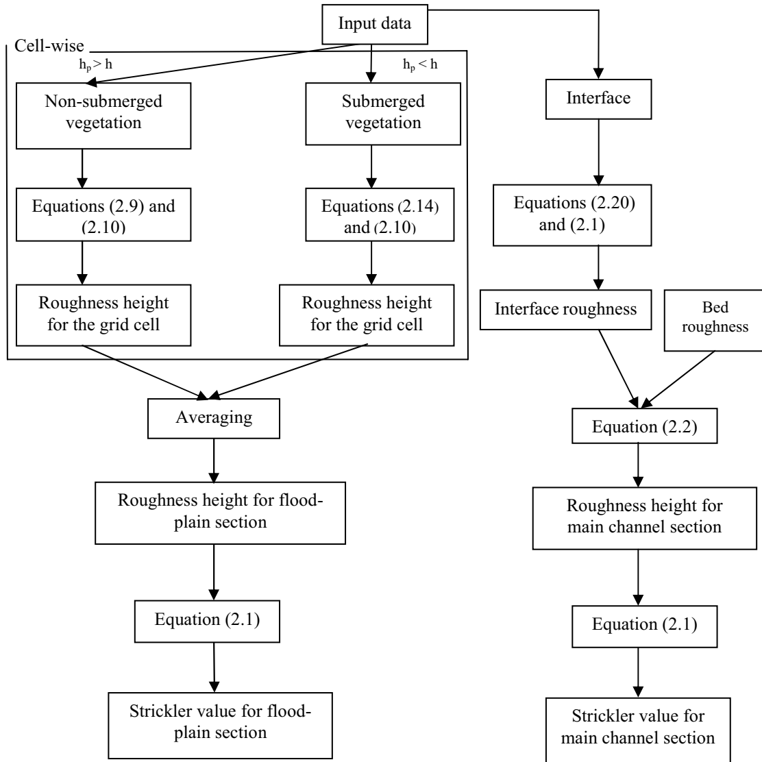
Figure 4-2: Algorithm of hydraulic-ecological model, i.e. calculation of Strickler value for each floodplain section
