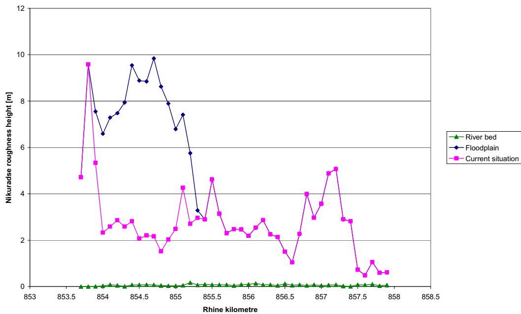
Figure 5-5: Roughness heights for each cross-section, forestation of all three areas (see section 3.2), HHQ of 1995
