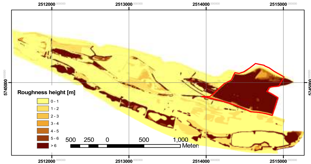
Figure 5-9: Roughness distribution over the floodplain, forestation behind the second summer dike (see section 3.2), HHQ of 1995, the red line shows the boundary of the forestation
