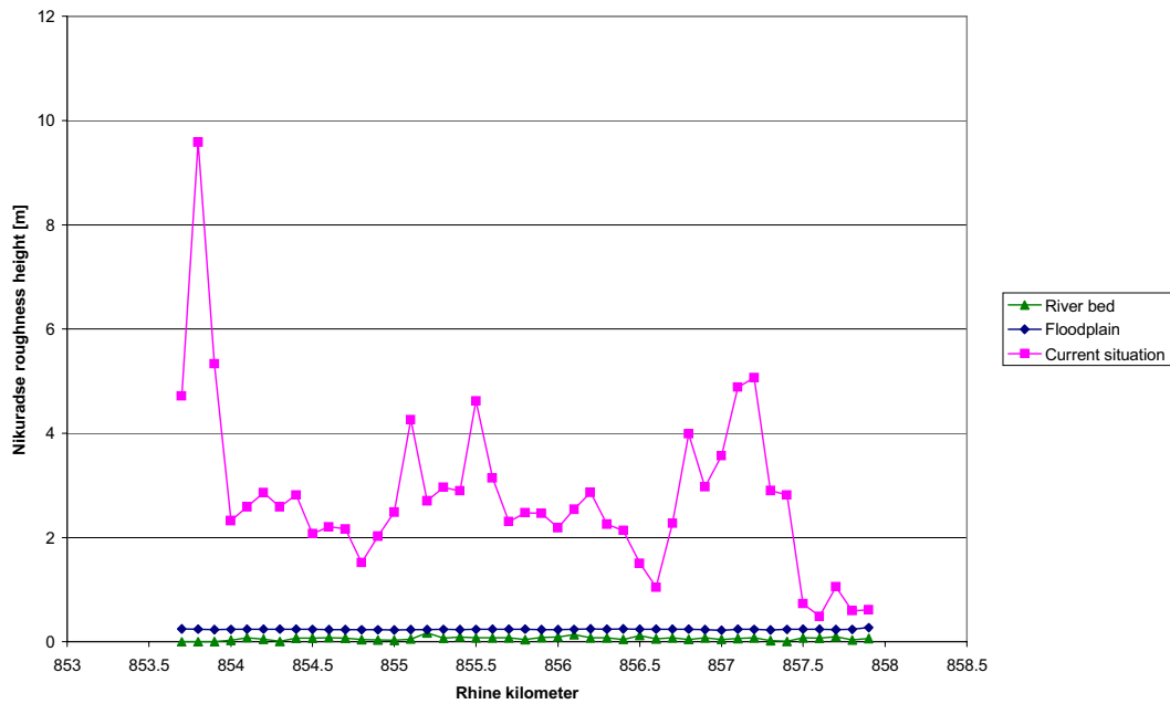
Figure 5-20: Roughness heights for each cross-section, grassland coverage (see section 3.2), HHQ of 1995
