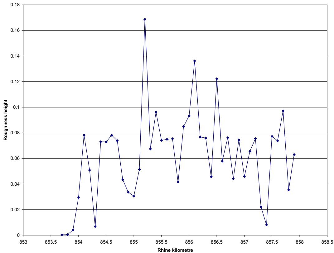
Figure 4-5: Calibrated floodplain roughness heights for each cross-section for the Rhine stretch along the Emmericher Ward
