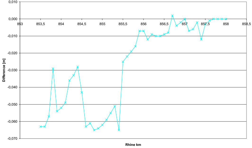
Figure 5-21: Differences in HHW between a scenario with a complete grassland coverage over the floodplain (see section 3.2) and the current situation
