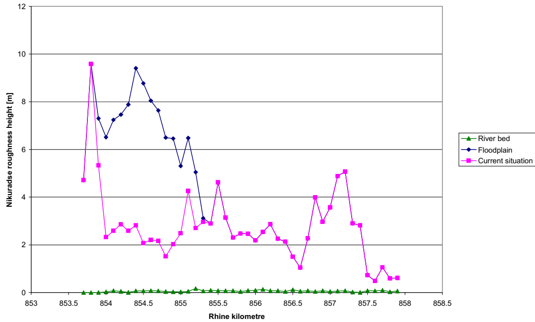
Figure 5-7: Roughness heights for each cross-section, forestation behind the first summer dike (see section 3.2), HHQ of 1995
