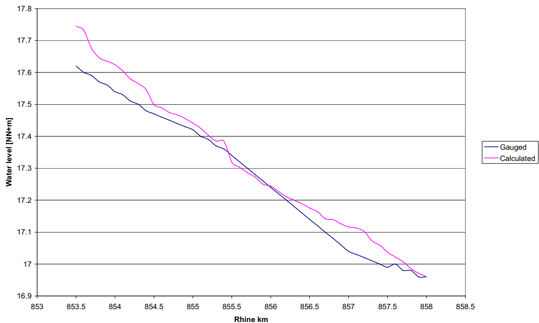
Figure 4-6: Comparison of gauged water levels and water levels that are calculated by FLYS for the Rhine stretch along the Emmericher Ward during the HHQ of 1995
