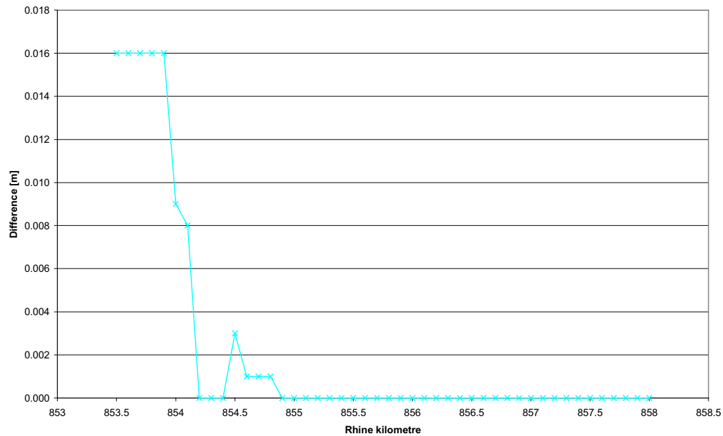
Figure 5-8: Differences in HHW between a scenario with forestation behind the first summer dike (see section 3.2) and the current situation
