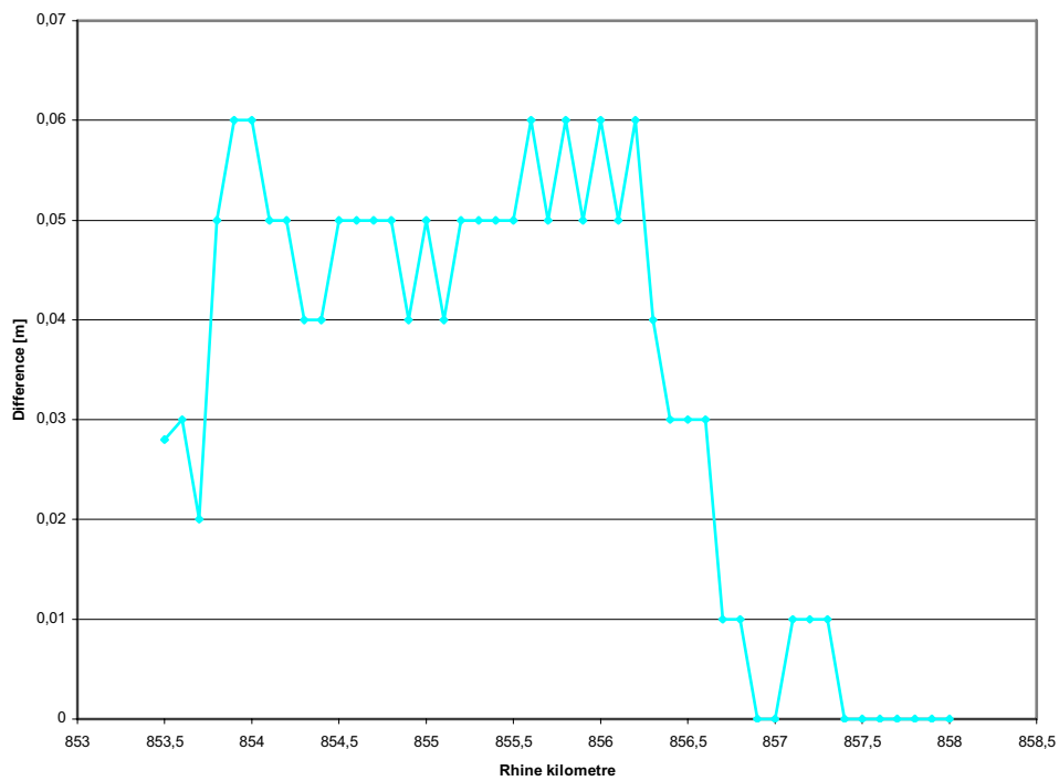
Figure 5-18: Differences in HHW between a scenario with complete coverage with PNV units and the current situation
