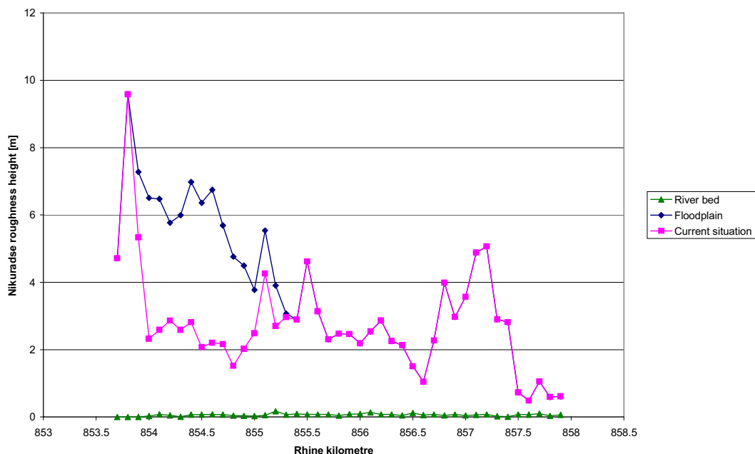
Figure 5-13: Roughness heights for each cross-section, forestation in clusters between both summer dikes (see section 3.2), HHQ of 1995
