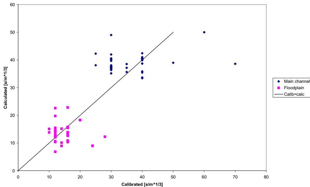
Figure 4-8: Calculated hydraulic roughness compared with calibrated values during the HHQ of 1995
