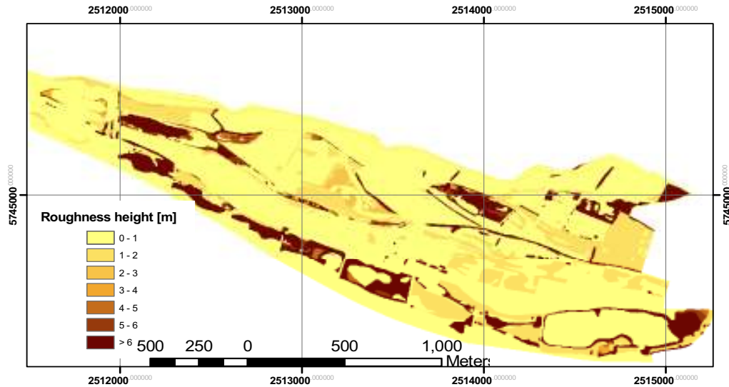
Figure 5-1: Roughness distribution over the floodplain during the HHQ of 1995
