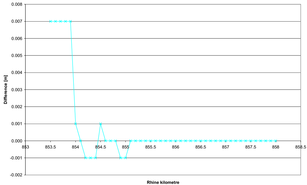
Figure 5-11: Differences in HHW between a scenario with forestation behind the second summer dike (see section 3.2) and the current situation
