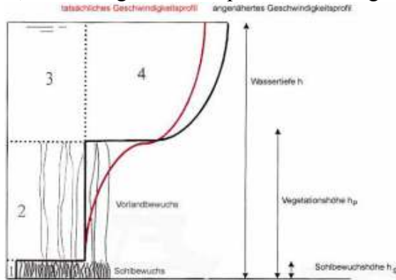
Figure 2-2: Velocity profile for submerged vegetation, the horizontal axis shows the flow velocity and the vertical axis shows the distance to the bed (Eisenhauer and Sommer, 2003)
