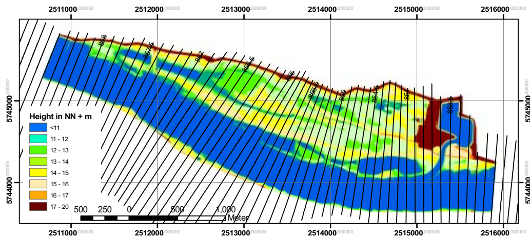
Figure 4-3: Digital elevation model Emmericher Ward
