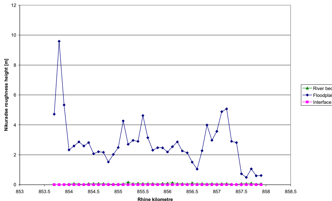
Figure 5-2: Roughness heights for each cross-section, current situation, HHQ of 1995
