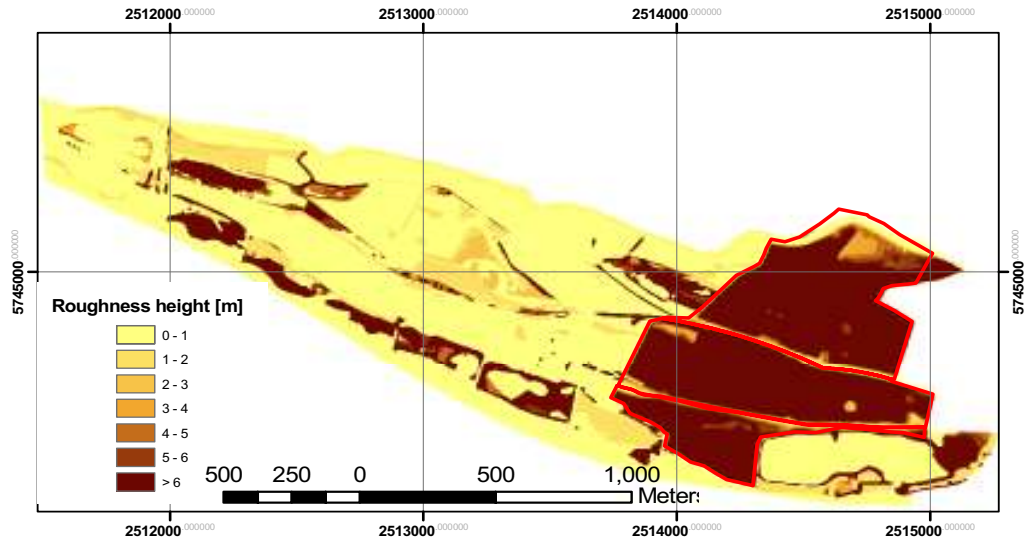
Figure 5-4: Roughness distribution over the floodplain, forestation of all three areas (see section 3.2), HHQ of 1995, the red line shows the boundary of the forestation
