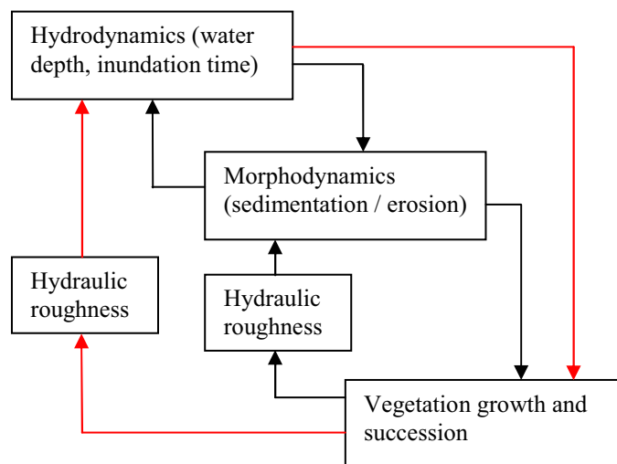
Figure 1-1: Relation between hydrodynamics and vegetation (Baptist et al., 2002)
