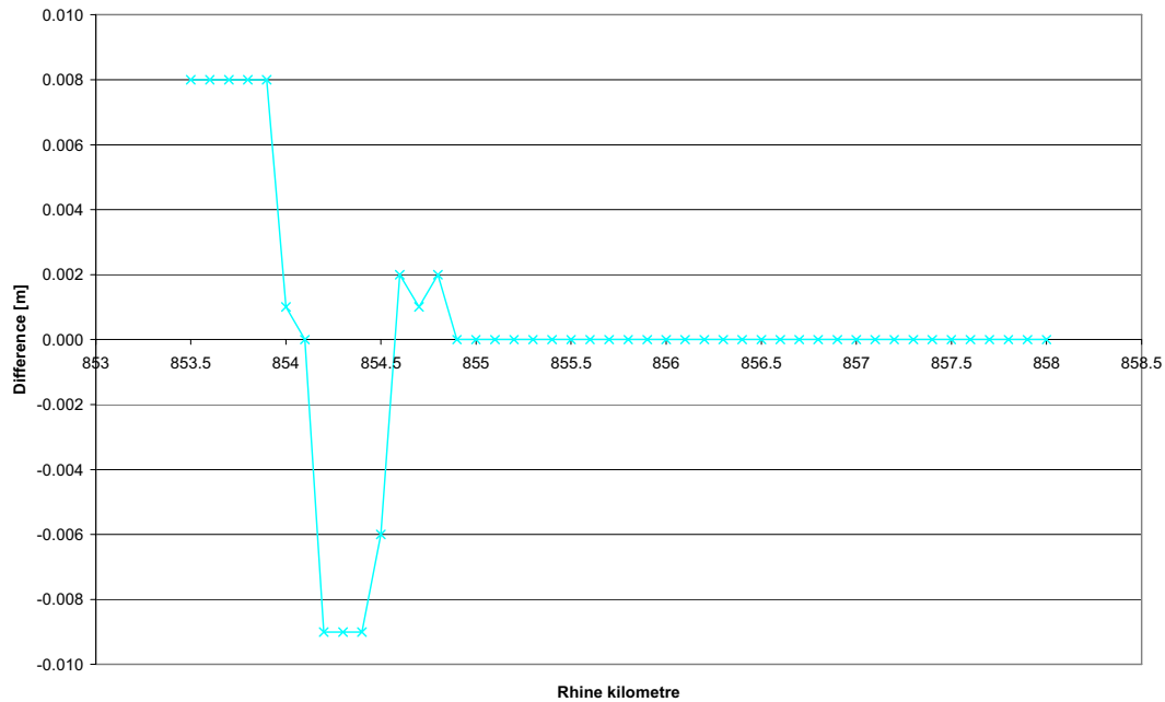
Figure 5-6: Differences in HHW between a scenario with forestation of all three areas (see section 3.2) and the current situation
