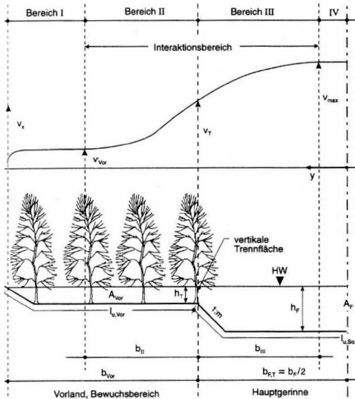
Figure 2-1: Subdivision of cross-section with fictive interface (Schumacher, 1995), the list of variables can be found on page 85
