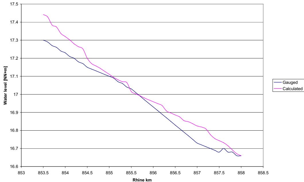
Figure 4-7: Comparison of gauged water levels and water levels that are calculated by FLYS for the Rhine stretch along the Emmericher Ward during the high-water discharge of 1993
