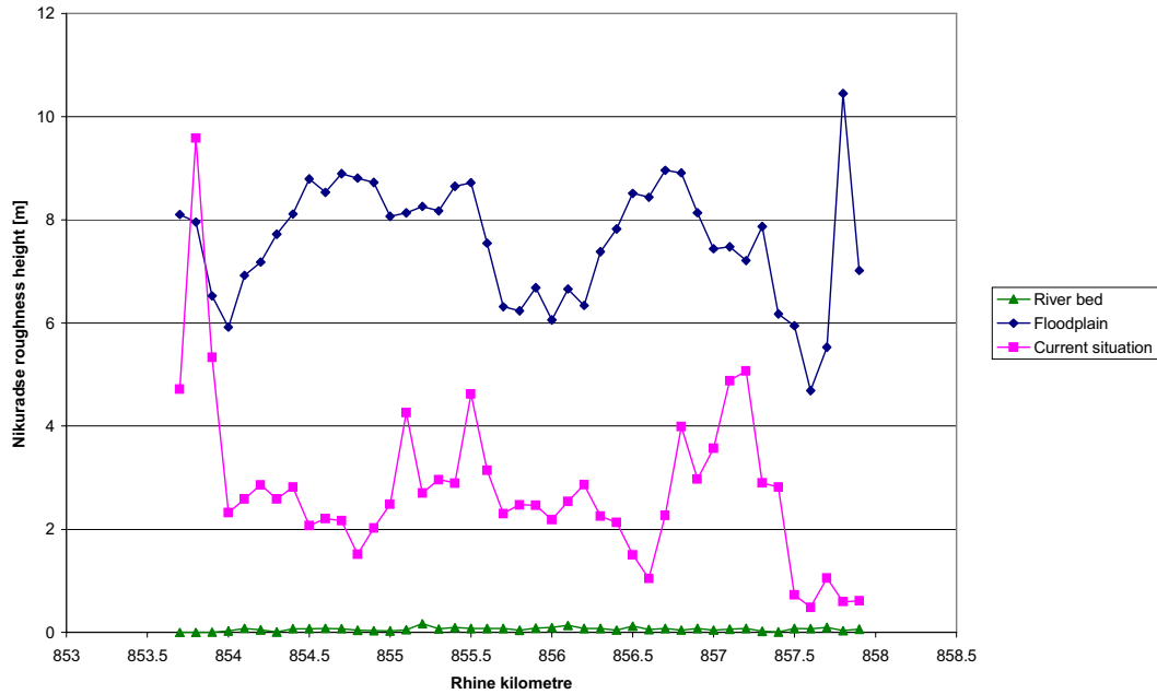
Figure 5-17: Roughness heights for each cross-section, complete coverage with PNV units, HHQ of 1995
