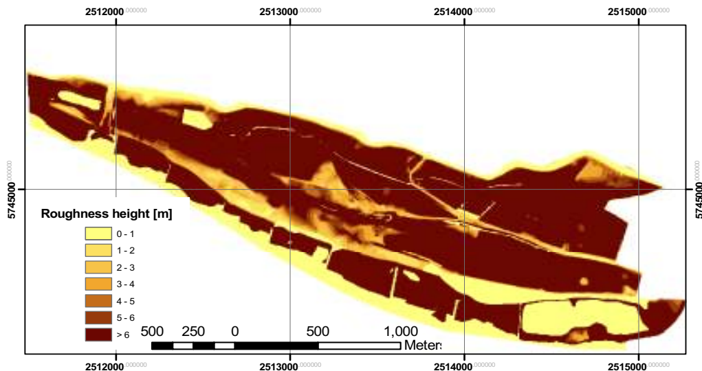
Figure 5-16: Roughness distribution over the floodplain in case of a coverage with PNV units, HHQ of 1995
