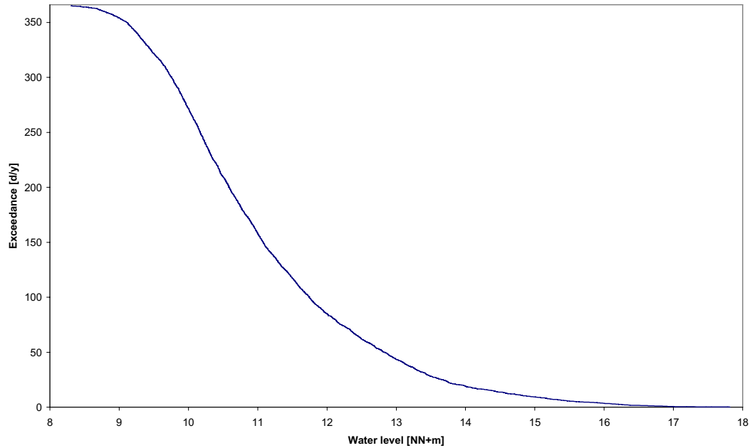
Figure 3-2: Mean number of days per year (vertical axis) that a water level (horizontal axis) was exceeded during the time period 1994 – 2003 at the gauge Emmerich
